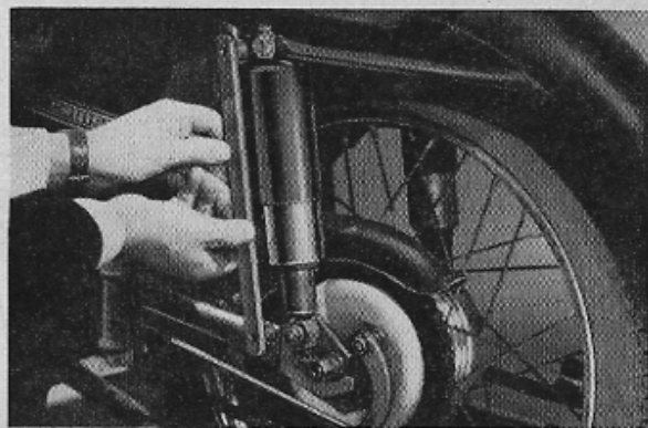
6875 Damper compressing tool for chain adjustment 5/-
