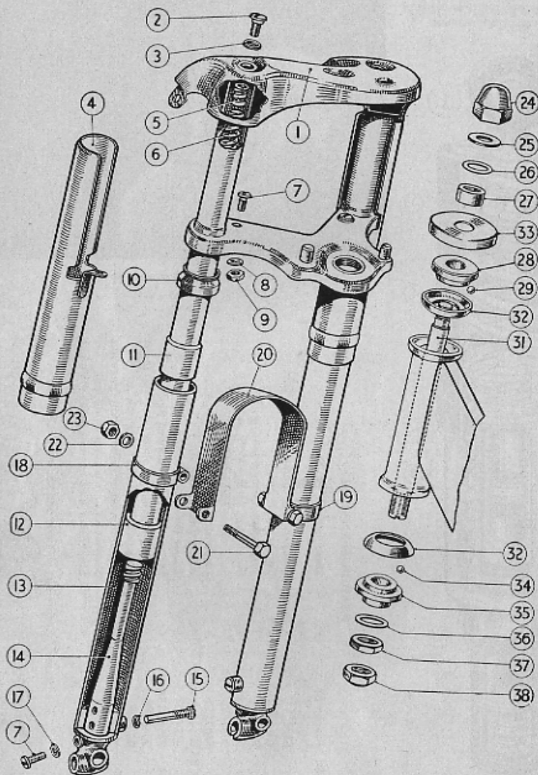
FRONT FORKS (CRUISER AND FALCON)
